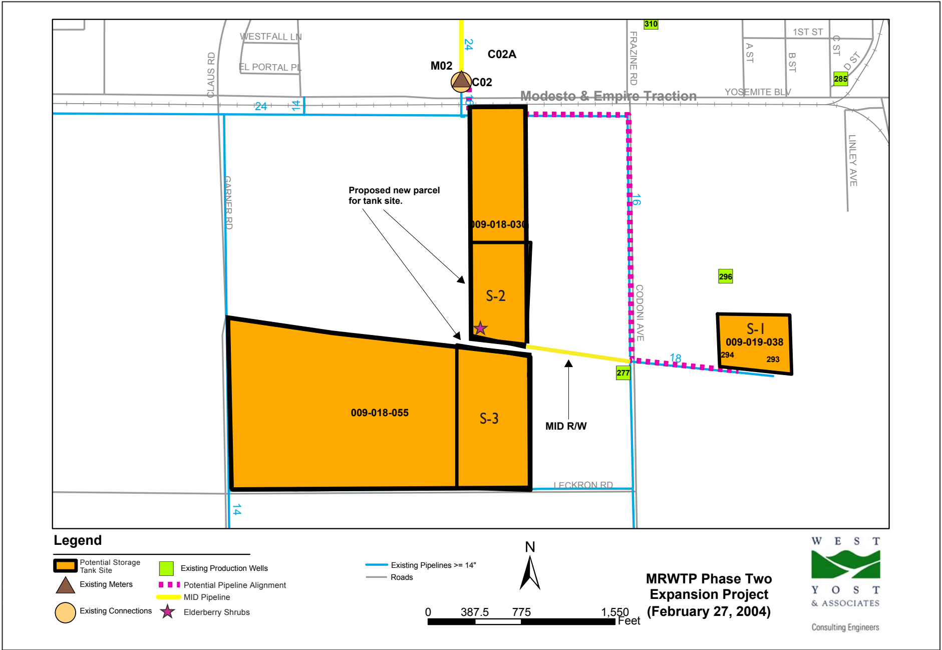
Figure 3.9-1 Location of Elderberry Shrubs and Valley Elderberry Longhorn Beetles
